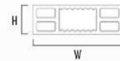
BPC-S150H50 (W: 150mm, H: 50mm)
