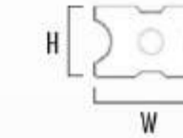
JOIST EU F40H25 (W: 40mm, H: 25mm)
