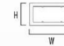
JOIST EU F60H30 (W: 60mm, H: 30mm)
